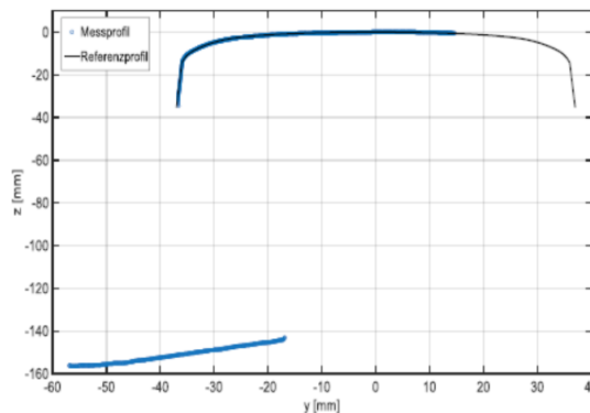
Measured profile aligned with a target profile; blue ... measured profile; black ... target profile
