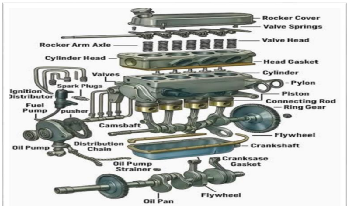
Fig 12.6 Important parts of I.C. Engine
