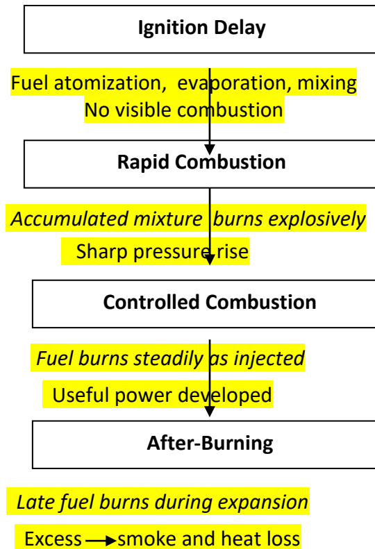
Fig 12.2 Stages of Combustion in a Four-Stroke Diesel Engine
