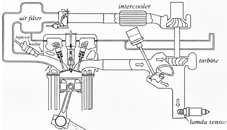
Fig 12.3 Air Intake System
