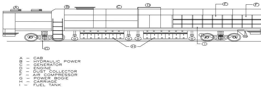
Fig.5.3 (RGM-72 Stone)
