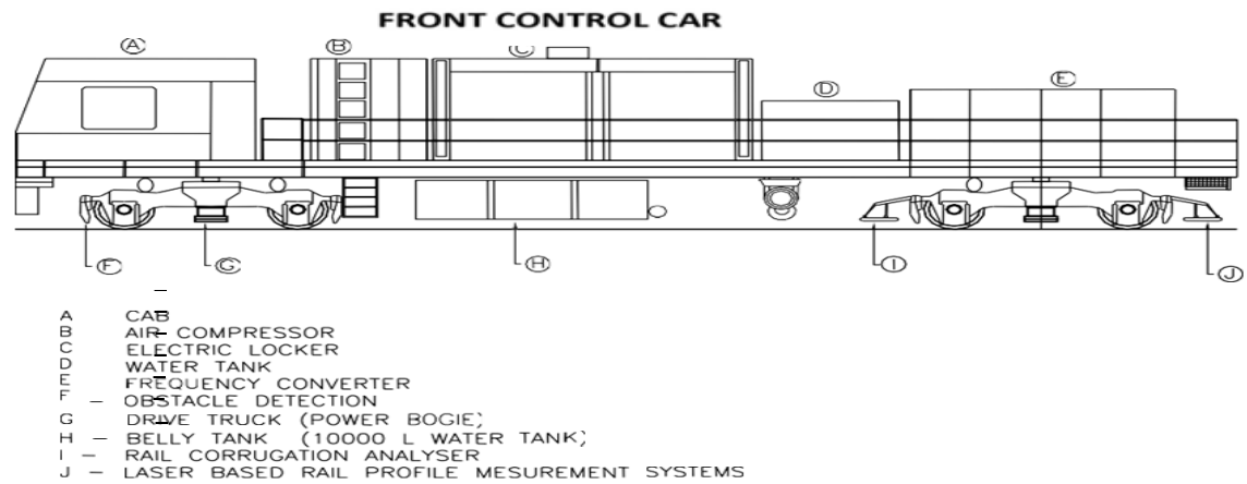
Fig. 5.2 (RGM-72 Stone)
