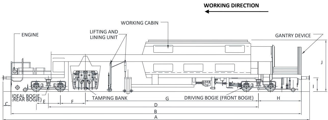
MULTIPURPOSE TAMPING (UNIMAT-COMPACT/M)
