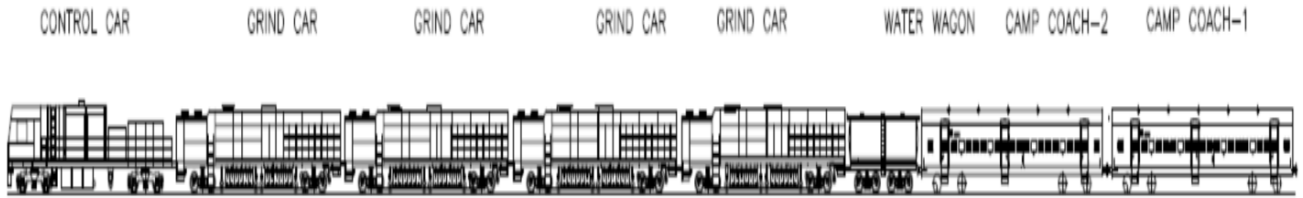
Fig. 5.1a (RGM-96 Stone)
