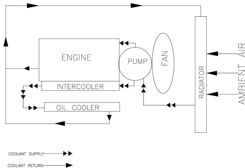
Fig 12.5 Cooling System
