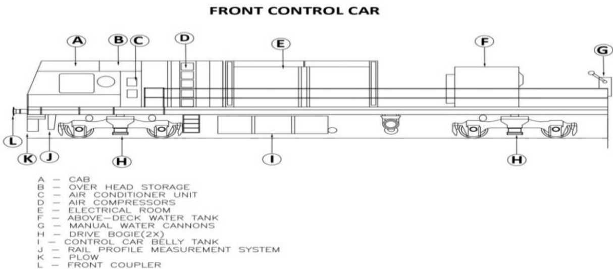
Fig.5.2a (RGM-96 Stone)
