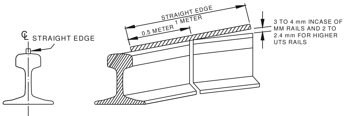
Fig.3.2 (c) Tolerances for Vertical Alignment at the Time of Welding
