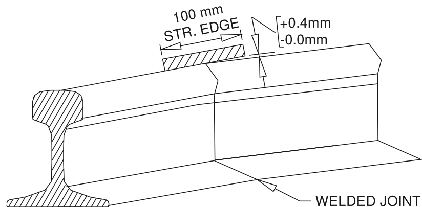
Fig. 3.3 (d) Tolerance for Finishing Top Table Surface of Welded Joint
