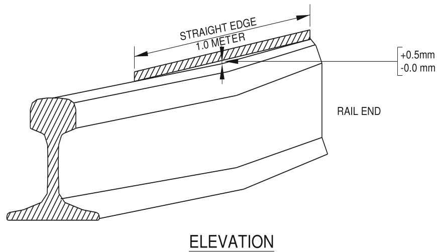
Fig. 3.1. (a) Tolerance on the End Bends in the Vertical Plane
