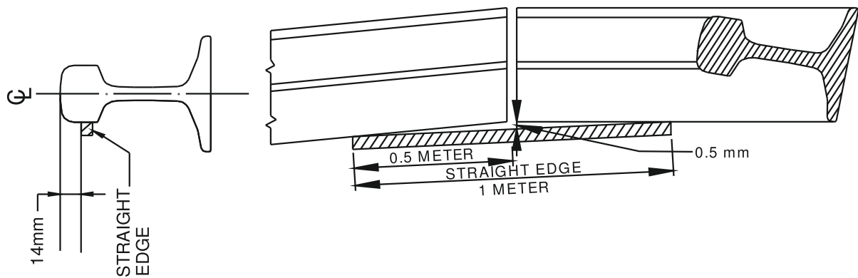
Fig. 3.2 (b) Tolerance for Lateral Misalignment at the Time of Welding
