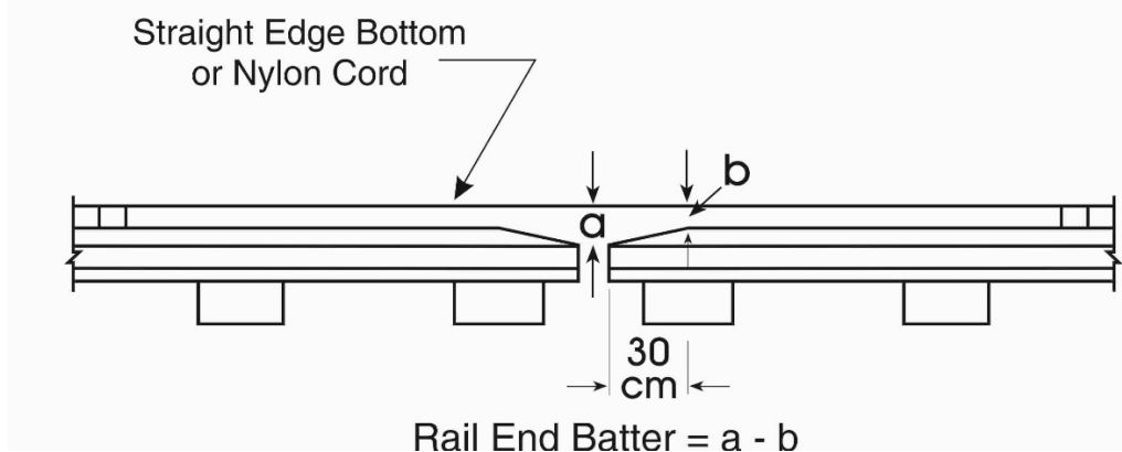
Rail End Batter – Method of Measurement
