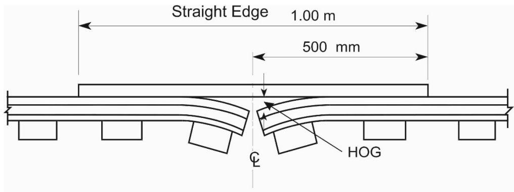
Hogging of Rail – Method of Measurement
