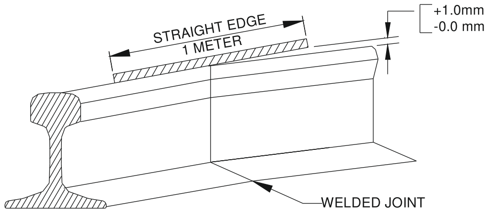
Fig. 3.3 (a) Tolerance for Vertical Misalignment of Welded Joint
