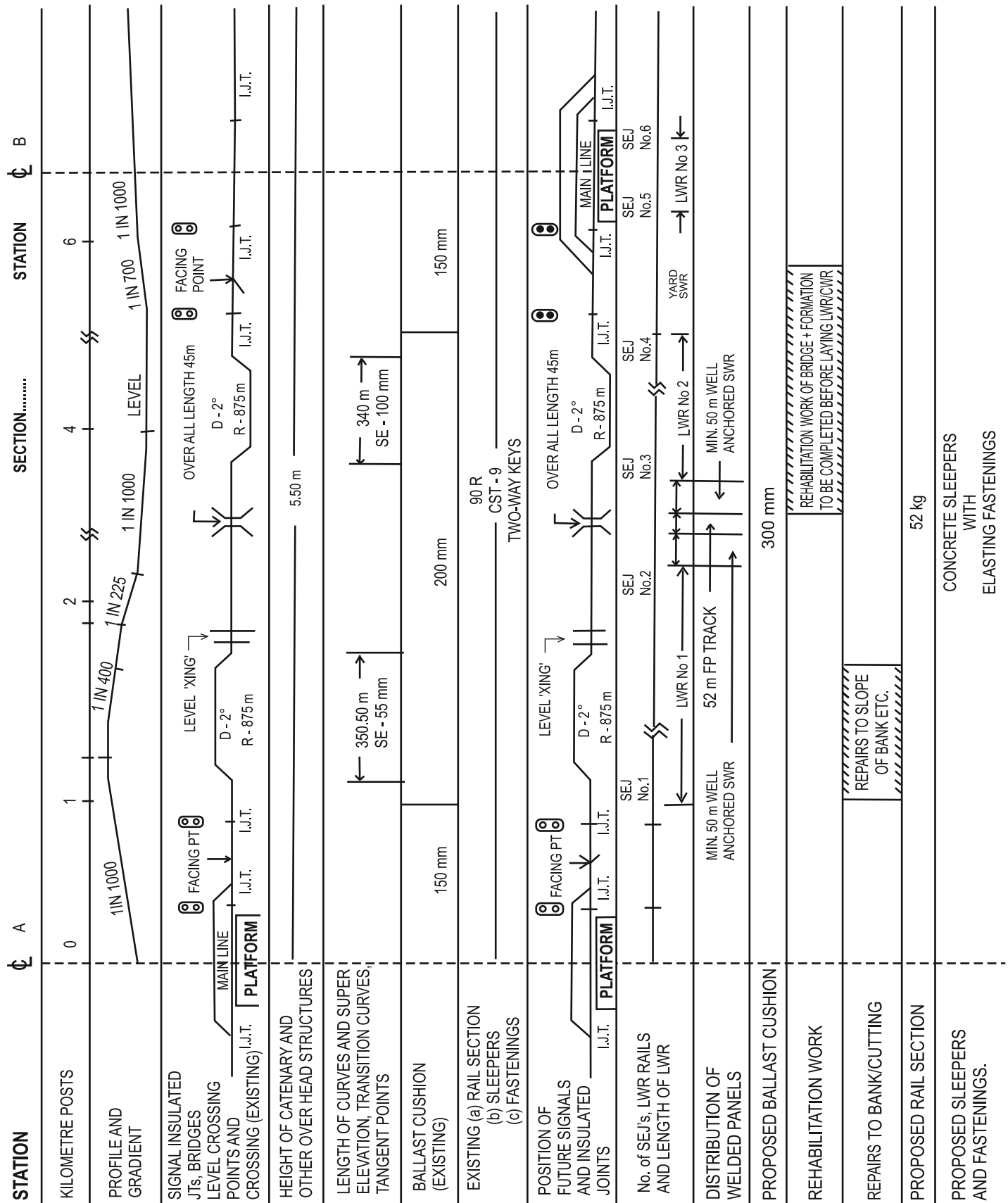
Fig 3.8 Proposal for laying LWR / CWR
