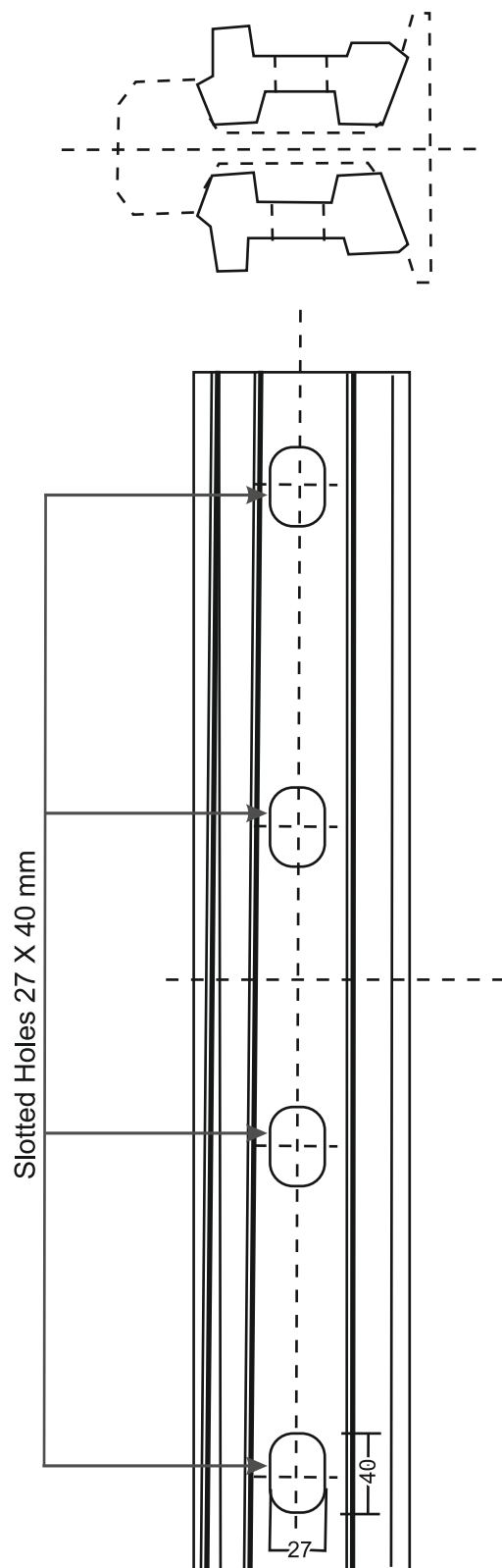
Fig. 3.13 SLOTTED FISH PLATE Back to Para 326(5) (e), 336
