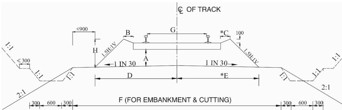
Ballast Profile (BG single line in embankment/cutting)
