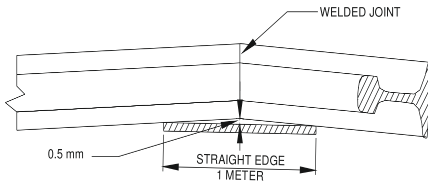
Fig. 3.3 (b) Tolerance for Lateral Misalignment of Welded Joint
