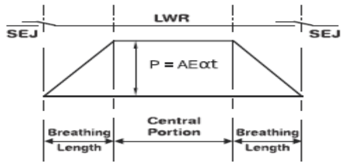
Fig. 3.5: Force Diagram in LWR / CWR
