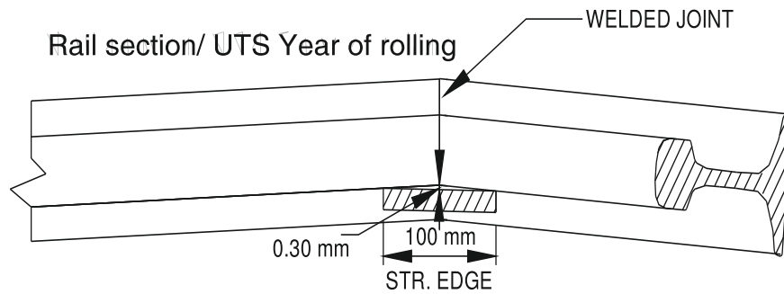
Fig. 3.3 (c) Tolerance for Finishing on Sides of Head of Welded Joint
