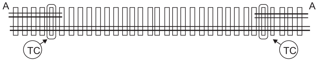
1. Removing of OHE rail Both the rails insulated for track circuiting
